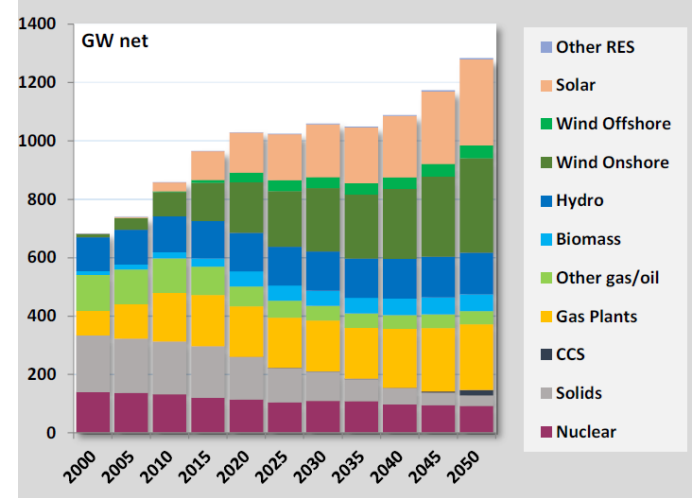
Operating power capacities
